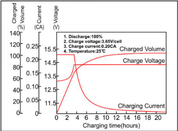
Constant voltage charging characteristics
